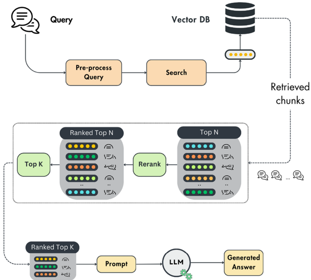
Figure 4.8: The re-ranking algorithm
