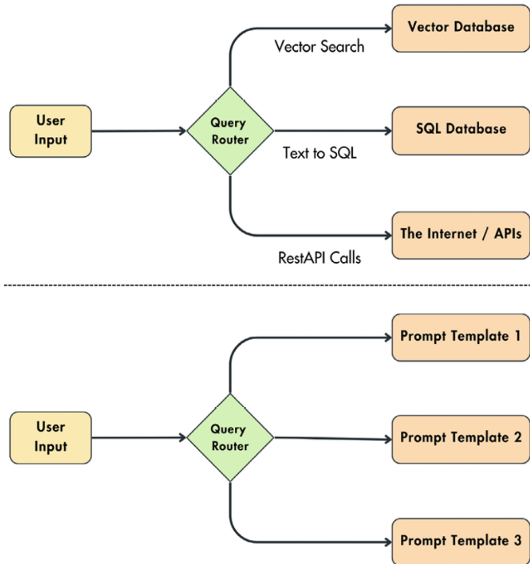
Figure 4.6: Query routing
