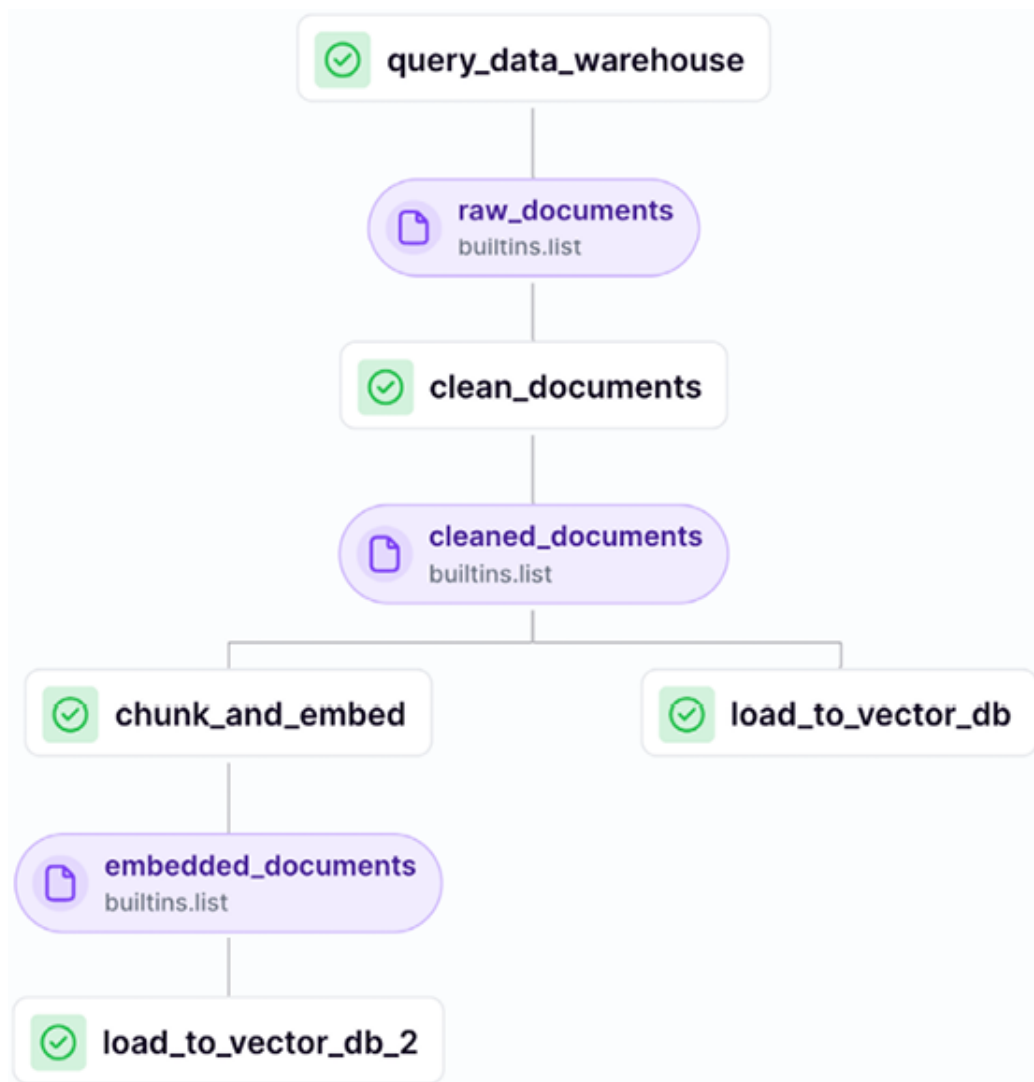
Figure 4.12: Feature pipeline DAG in the ZenML dashboard
