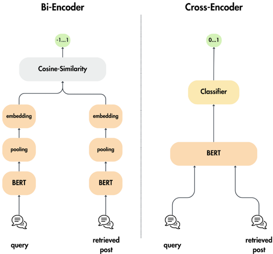
Figure 4.7: Bi-encoder (the standard embedding model) versus cross-encoder
